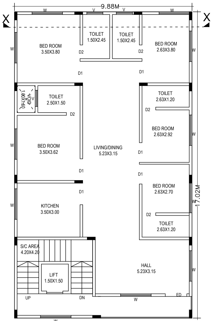
TYPICAL FIRST & SECOND FLOOR PLAN
